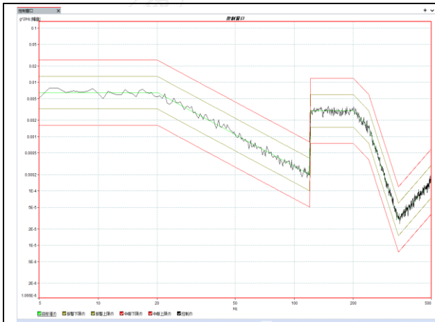
Fig.2-7 Road transport vibration test curve (Y-axis)
